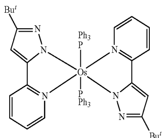
Os(bppz) 2 (PPh 3 ) 2
